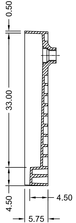
SECTION B-B
