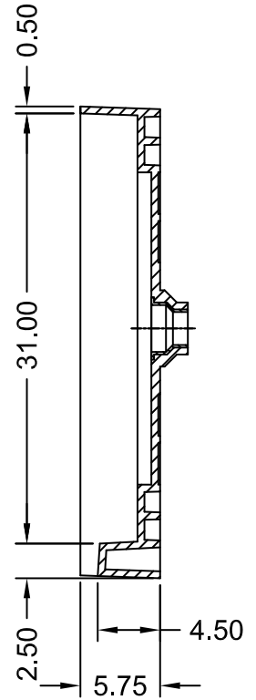
SECTION B-B
