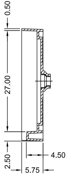
SECTION B-B
