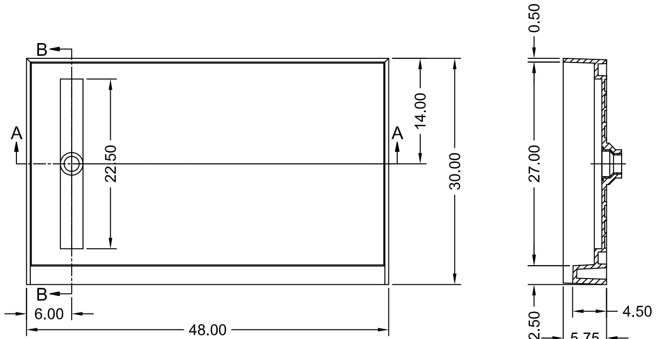
SECTION B-B
